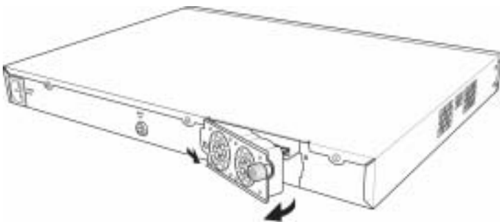
Figure 55. Removing the fan module
